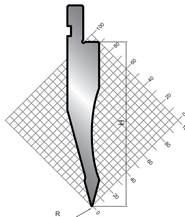
mod. S1996 (HR) 30°
